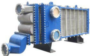
Wide Gap Welded Plate Heat Exchanger (without gaskets between plates)
